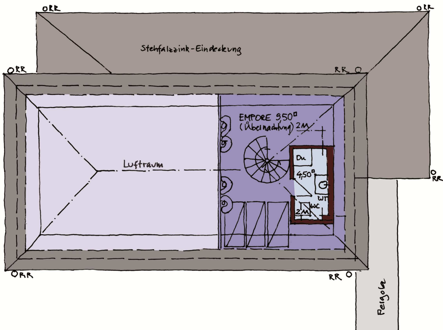
Grundriss EMPORE
